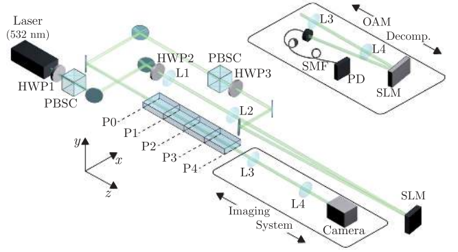
FIG. 3. Experimental setup. Lenses L1 and L2 expand the 532-nm laser beam. An SLM creates a diffraction grating with variable combinations of OAM \ell = +1 and \ell = -1 . The first-order diffraction is weakly focused ( f \sim 2 \text{ m} ) onto the entrance facet ( P0 ) of a set of four 10\text{-cm} \times 4\text{-cm} \times 0.5\text{-cm} glass slabs. HWP2 is used to vary the SLM diffraction efficiency. HWP3 and PBS provide additional control of P_0 . The beam intensity profile is imaged at the entrance facet P0 and at the exit facet of each glass plate P1 – P4 . The M = 6 imaging system is fixed with respect to the camera and translated as a single entity. The camera can be replaced with an SLM and single-mode fiber to perform an OAM decomposition.
