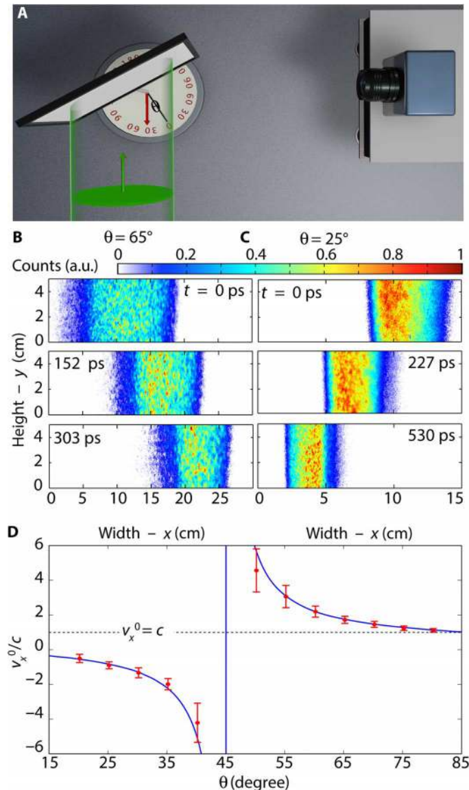
Fig. 2. Time order inversion. (A) A sketch of the experiment. A plane wavefront (green) impinges on a tilted screen, and the scattered radiation is recorded at 90^\circ with a time-resolving intensified charge-coupled device (iCCD) camera. Changing the angle \theta between the input wave and the screen allows a change in the scattering source velocity component along the camera/observer direction. (B) Three snapshots acquired by the camera at three different times for an incident angle ( \theta = 65^\circ ) such that the scattering speed toward the camera is subluminal. In this case, the time order is maintained and the perceived source moves from left to right (full video available as Supplementary_Video_1.mp4). (C) For \theta = 25^\circ , the source velocity toward the detector is superluminal and event time ordering is reversed; that is, the same wavefront measured in (B) is now seen as propagating in the opposite direction, from right to left (full video available as Supplementary_Video_2.mp4). (D) The measured speed along the x direction (red dots) compared with the theoretical prediction (blue curve).
